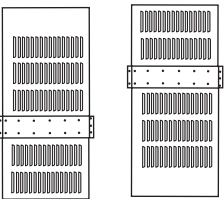
Detail of radiator header enlarged 3 times
